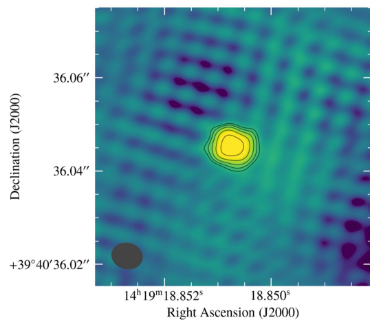
The measured source size, from the high-resolution 1.6 GHz EVN image, confirmed non-thermal emission and revealed FIRST J1419+3940 as an orphan long gamma-ray burst afterglow (Marcote et al. 2019, ApJL, 876, L14).
